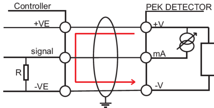
Source wiring
